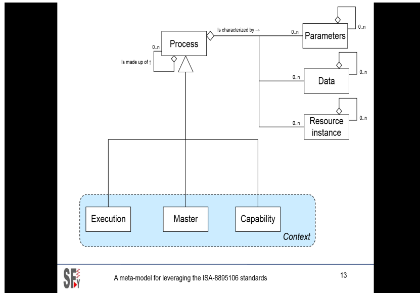
Fig. . Process Meta-model
