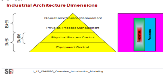
Fig. . Meta-model reification
