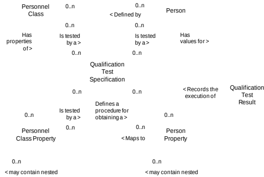
Fig . ISA-95 Personnel model
