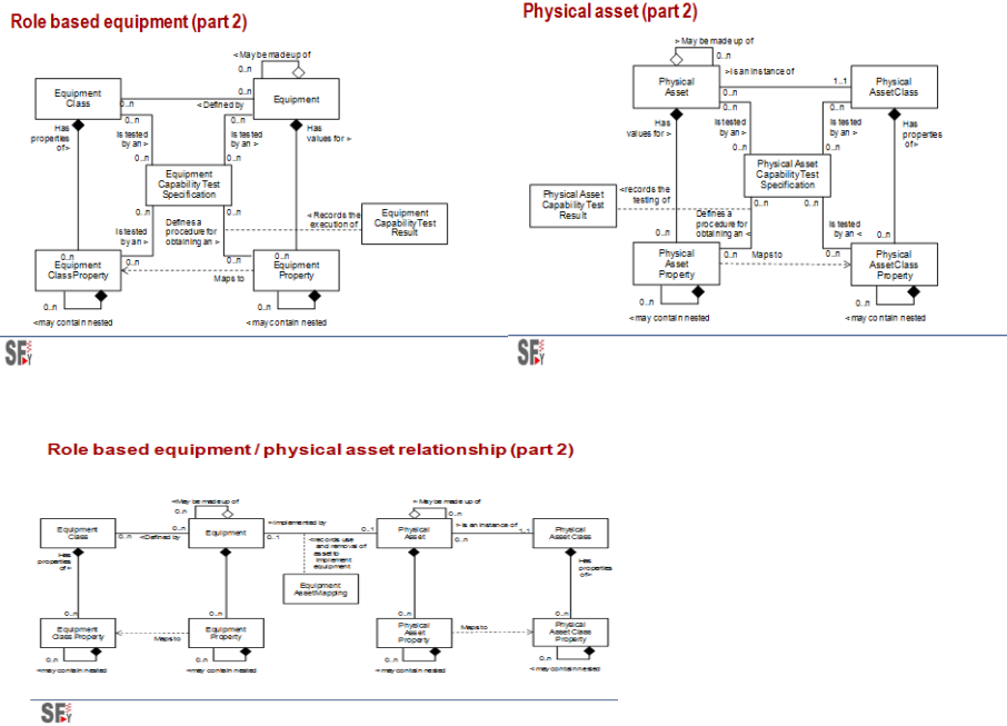
Fig. . Table . Figure ISA-95 Equipment models
